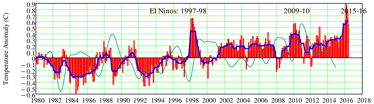
7A. Satellite Global Temp Anomaly, 13 Month Avg (Blue), and Southern Oscillation Index, SOI - (Green)
